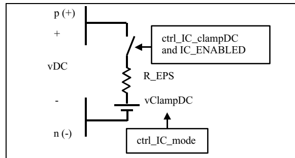
Figure 3. Capacitor static model.
